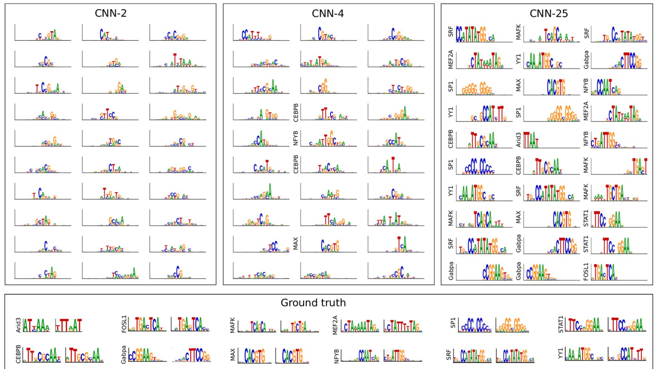
Fig 2. Comparison of first layer filters for CNNs with a different max-pool size. Sequence logos for first convolutional layer filters are shown for CNN-2 (Left), CNN-4 (Middle), and CNN-25 (Right). The sequence logo of the ground truth motifs and its reverse complement for each transcription factor is shown at the bottom. The y-axis label on select filters represents a statistically significant match to a ground truth motif.
