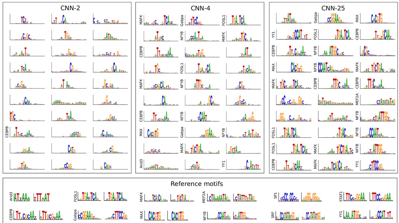
Fig 4. Comparison of the first layer filters for CNNs trained on in vivo sequences. Sequence logos for first convolutional layer filters are shown for CNN-2 (Left), CNN-4 (Middle), and CNN-25 (Right). The sequence logos of reference motifs and their reverse complements for each transcription factor from the JASPAR database is shown at the bottom. The y-axis label on select filters represent a statistically significant match to a reference motif.
