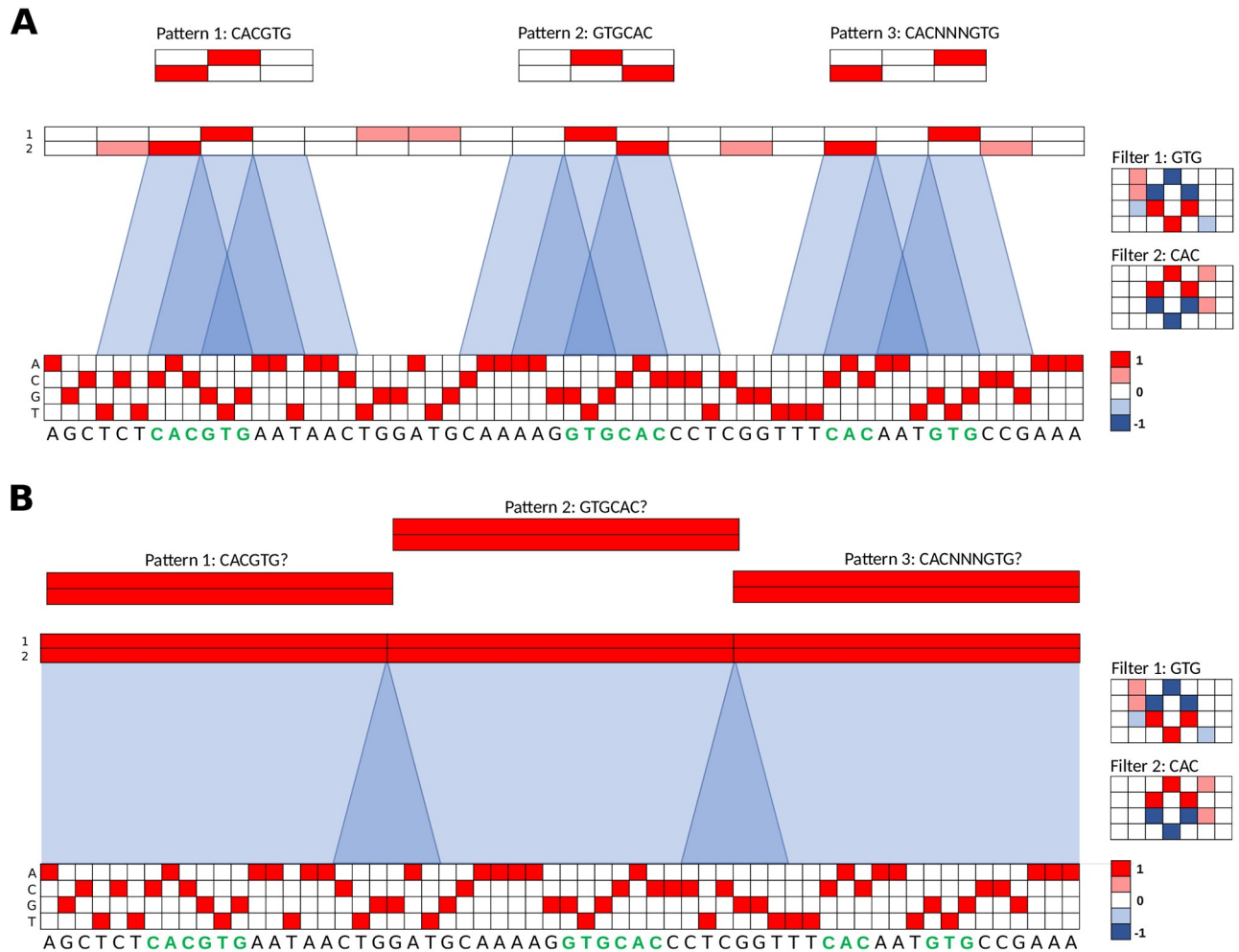
Fig 1. Toy model for representation learning of sequence motifs. (A,B) An example 60 nt one-hot encoded sequence contains 3 patterns (shown in green): CACGTG, GTGCAC, and CACNNGTG. Two filters, each of length 7 (7 columns and 4 rows, one for each nucleotide), are shown to the right. A partial motif representation has been captured by each filter: GTG for filter 1 (Top) and CAC for filter 2 (Bottom). The max-pooled feature maps are shown above the sequence. The feature maps have the same size as the sequence by adding 3 zero-padding units to each end of the sequence prior to convolution (not shown in diagram). (A) Shows the feature maps when employing a small max-pooling size of 3, which creates overlapping receptive fields, highlighted in blue. 3 second layer convolutional filters, shown above, demonstrate a feature map pattern that can resolve each embedded sequence pattern. (B) Shows the feature maps when employing a larger pooling size of 20 using the same filters as (A). The larger receptive fields have a large spatial uncertainty along with a small overlap in receptive fields from neighboring neurons. Each of the 3 second layer convolutional filters, shown above, is unable to find a unique feature map pattern that can resolve any embedded sequence pattern.
