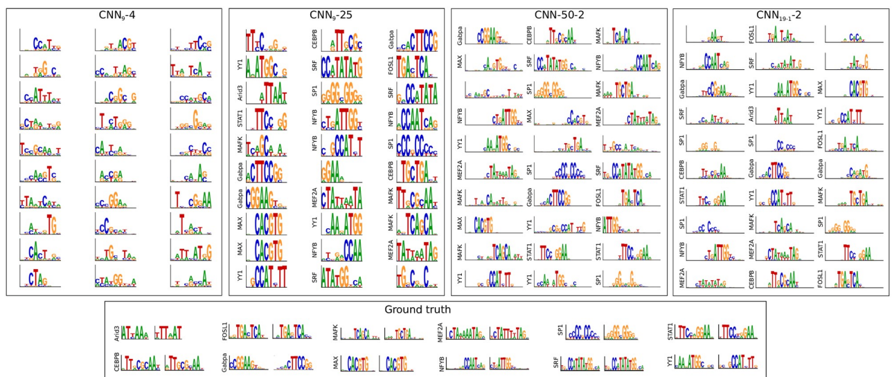
Fig 3. Representations learned by first layer filters for alternative CNN architectures. Sequence logos for first convolutional layer filters are shown for (from left to right): CNN 9 -4, CNN 9 -25, CNN 50 -2, and CNN 19 -2. The sequence logo of the ground truth motifs and its reverse complement for each transcription factor is shown at the bottom. The y-axis label on select filters represent a statistically significant match to a ground truth motif.
