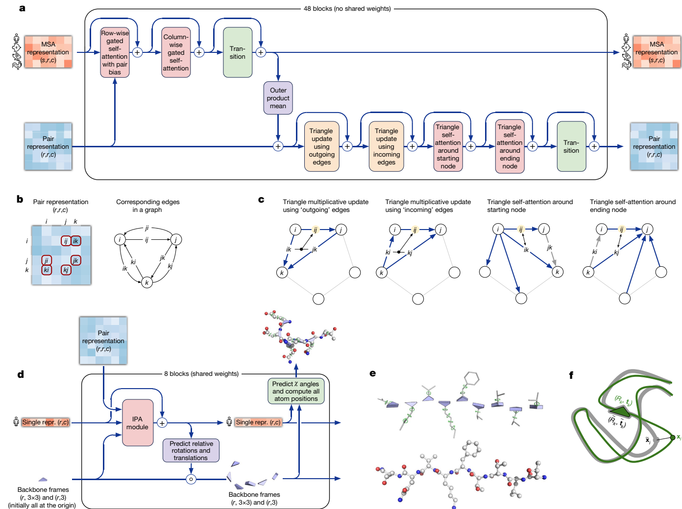
Fig. 3 | Architectural details. a, Evoformer block. Arrows show the information flow. The shape of the arrays is shown in parentheses. b, The pair representation interpreted as directed edges in a graph. c, Triangle multiplicative update and triangle self-attention. The circles represent residues. Entries in the pair representation are illustrated as directed edges and in each diagram, the edge being updated is ij . d, Structure module including Invariant point attention (IPA)
